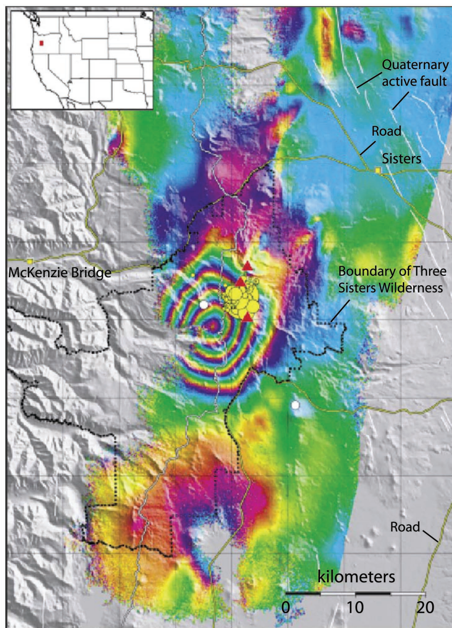
Figure B6. Interferogram from InSAR imaging process showing the area of uplift (1997–2001) at the Three Sisters volcanoes (red triangles) in the Cascade Range in central Oregon, USA (circles show locations of earthquakes). (Photograph modified from Reference 41.)
